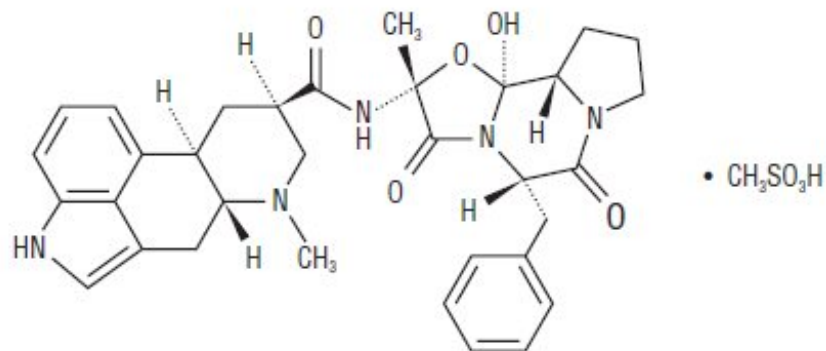
Dihydroergotamine mesylate C 33 H 37 N 5 O 5 •CH 4 O 3 S Mol. wt. 679.80
